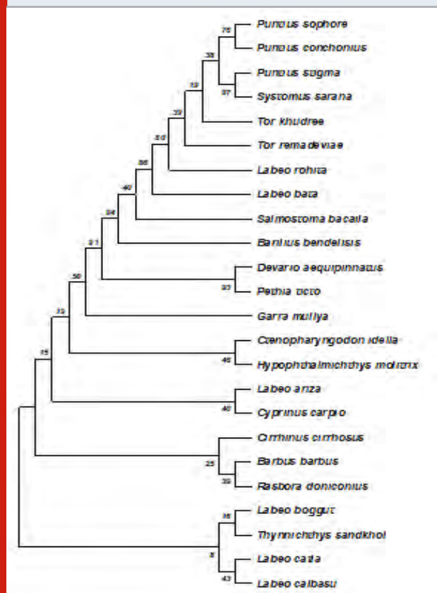
Figure 3: C-Cytosine
