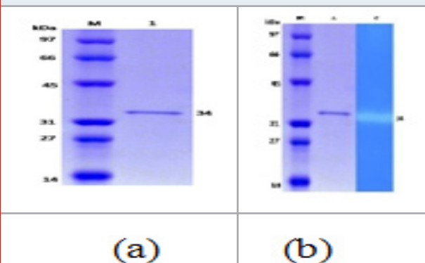
Figure 1.b: Keratinase Zymogram
